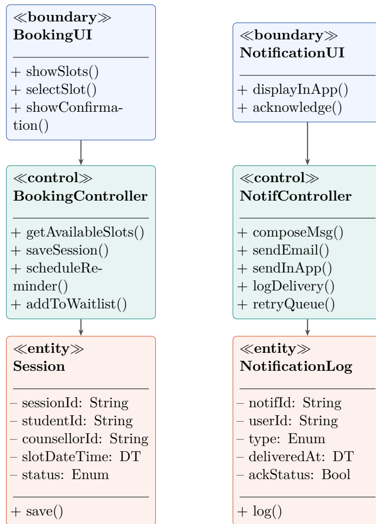
Figure 15: Analysis Class Diagram — UC-05 &amp; UC-06
