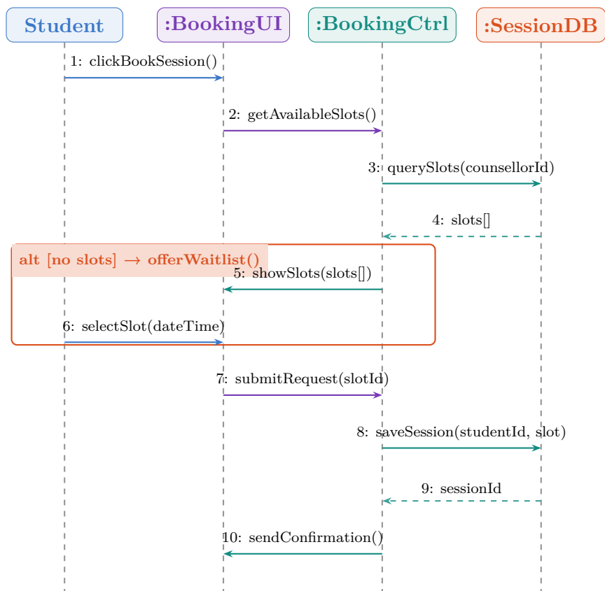
Figure 11: Sequence Diagram — UC-05: Request Counselling Session
