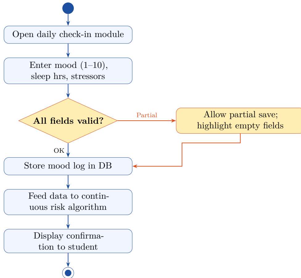
Figure 8: Activity Diagram — UC-03: Log Daily Mood
