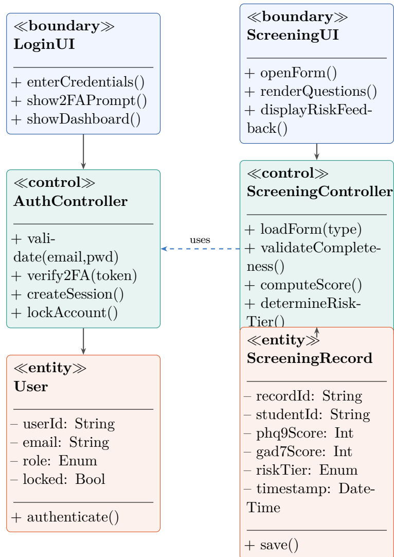
Figure 5: Analysis Class Diagram — UC-01 &amp; UC-02
