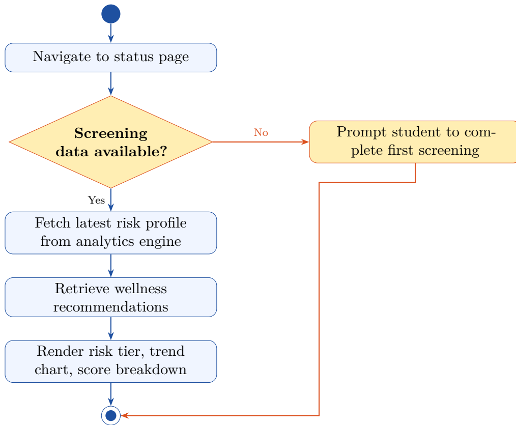
Figure 9: Activity Diagram — UC-04: View Mental Health Status
