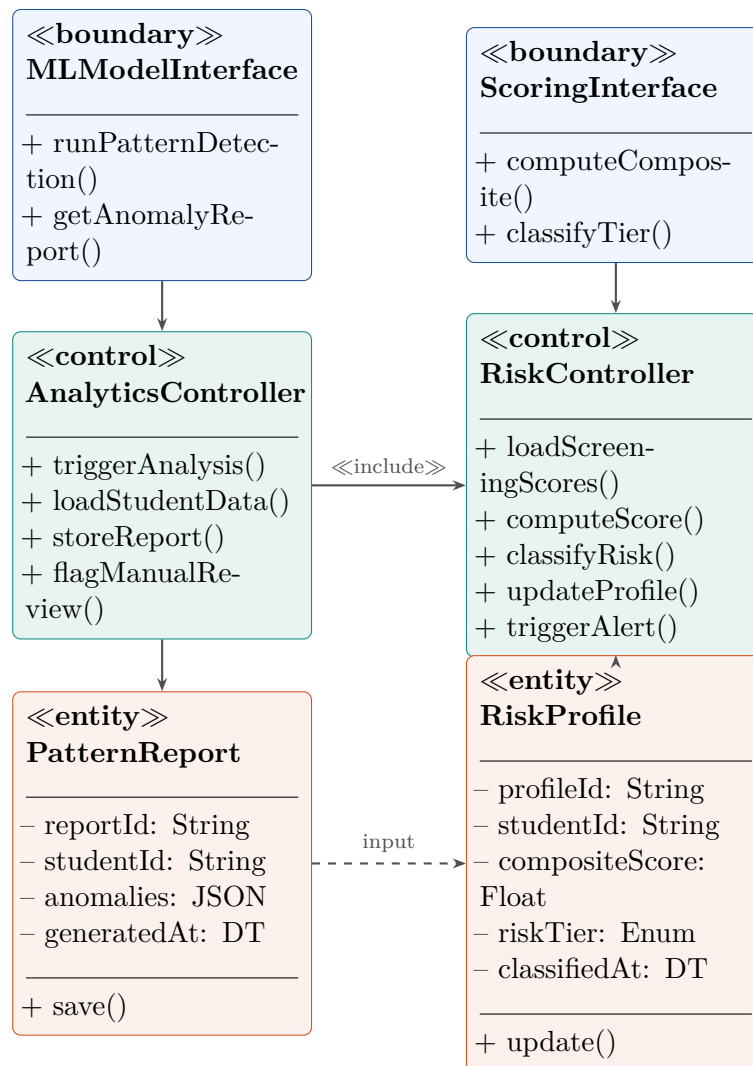
Figure 25: Analysis Class Diagram — UC-09 &amp; UC-10
