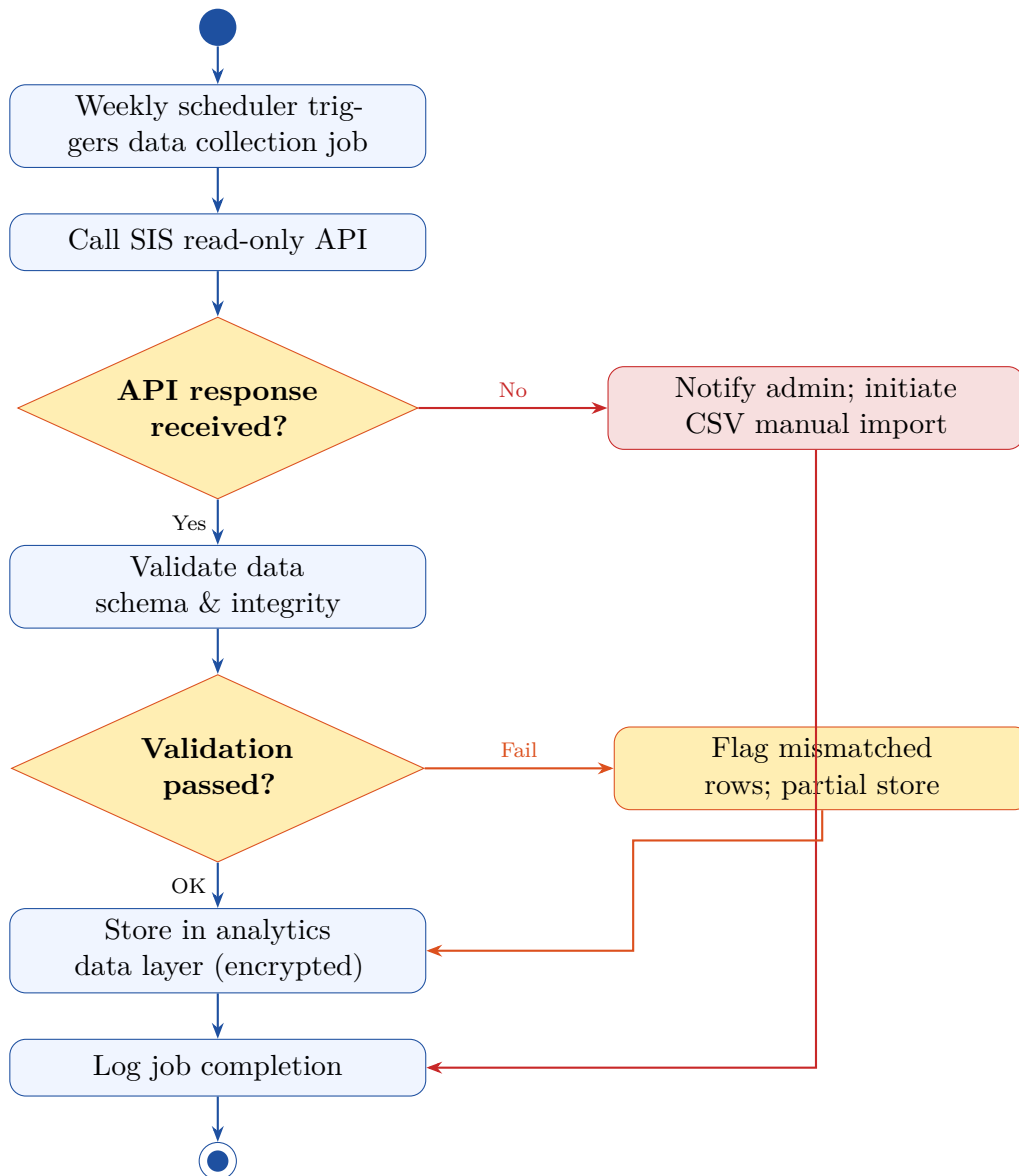
Figure 19: Activity Diagram — UC-08: Collect Student Data
