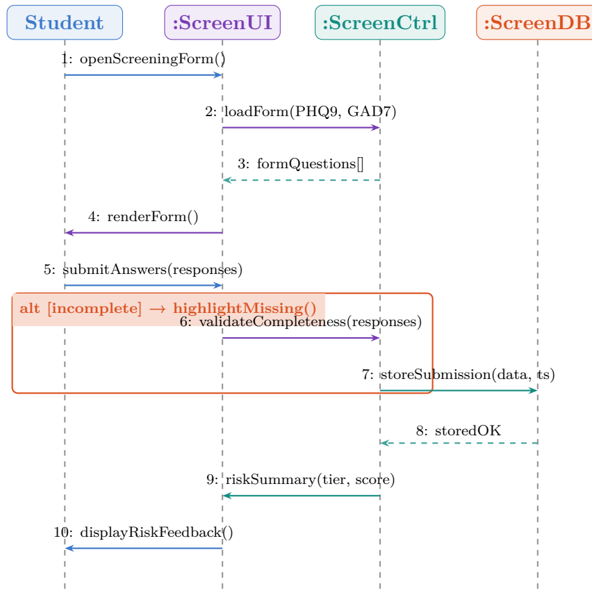
Figure 2: Sequence Diagram — UC-02: Fill Standardised Screening
