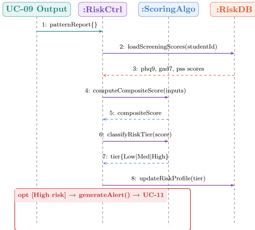
Figure 22: Sequence Diagram — UC-10: Detect Mental Health Risk
