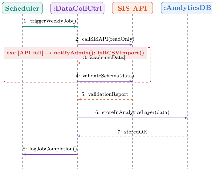
Figure 17: Sequence Diagram — UC-08: Collect Student Data
