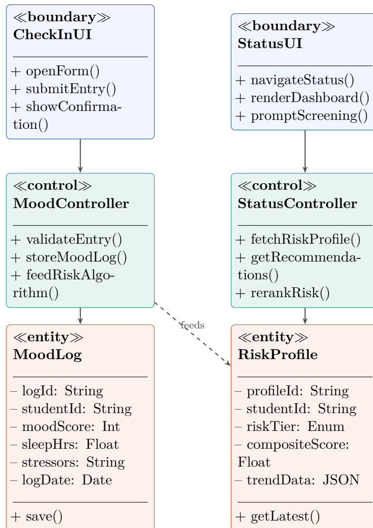
Figure 10: Analysis Class Diagram — UC-03 &amp; UC-04
