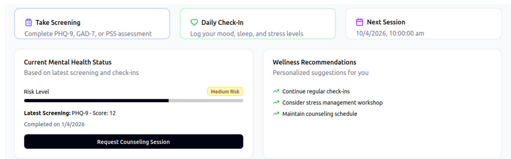
Figure 29: UI-04 — Student Mental Health Status Dashboard (UC-04)
