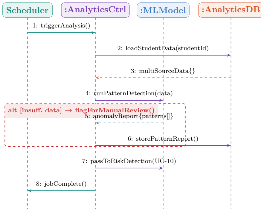
Figure 21: Sequence Diagram — UC-09: Analyse Behavioural Patterns
