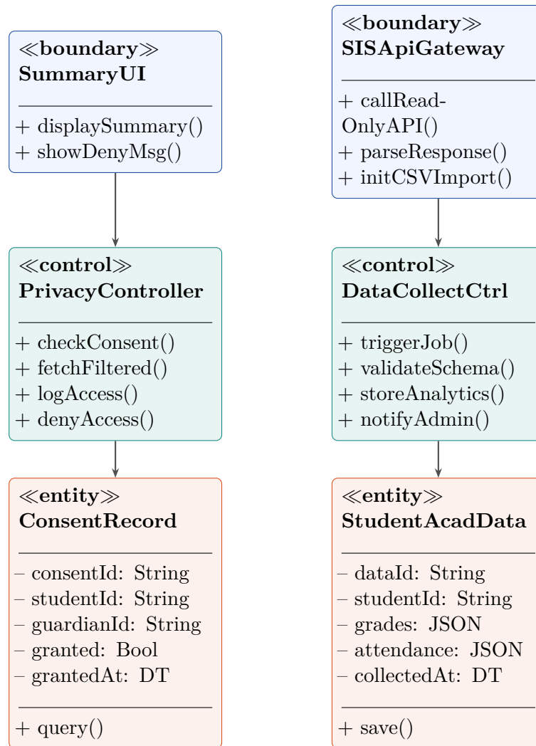
Figure 20: Analysis Class Diagram — UC-07 &amp; UC-08
