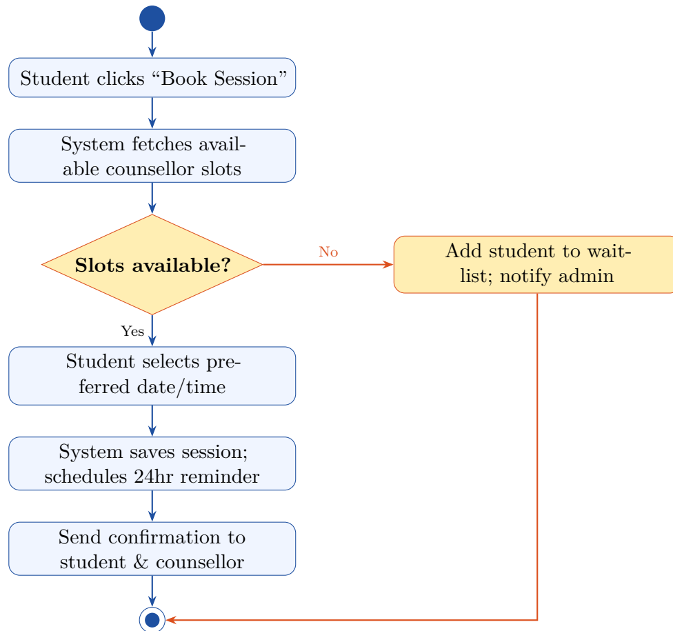
Figure 13: Activity Diagram — UC-05: Request Counselling Session
