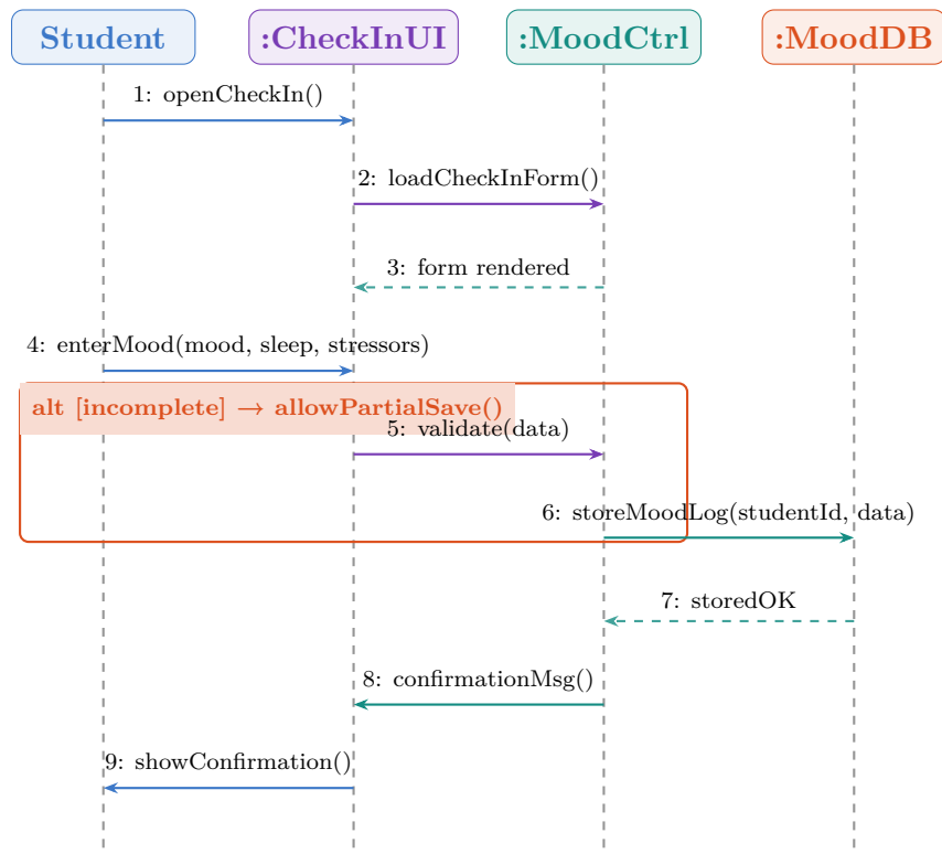
Figure 6: Sequence Diagram — UC-03: Log Daily Mood
