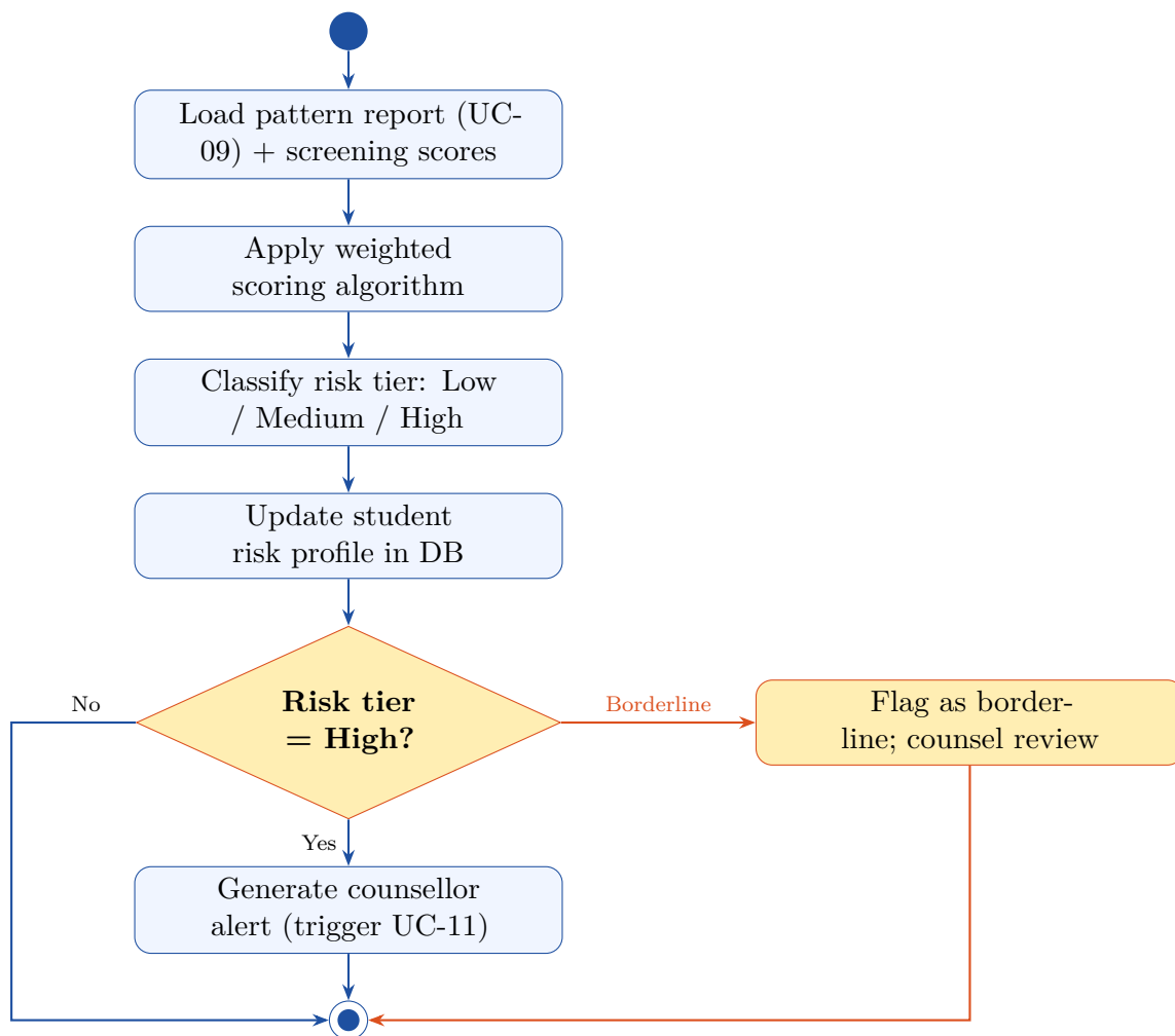
Figure 24: Activity Diagram — UC-10: Detect Mental Health Risk
