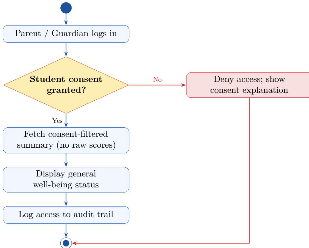
Figure 18: Activity Diagram — UC-07: View Well-being Summary
