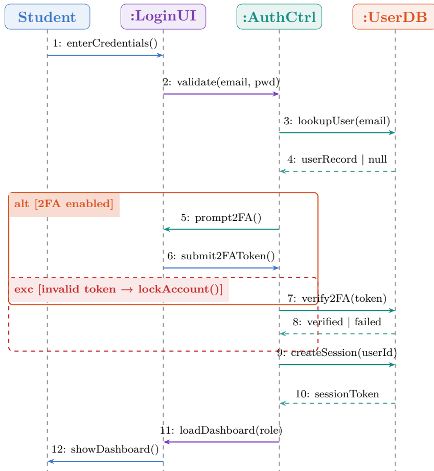
Figure 1: Sequence Diagram — UC-01: Register / Login
