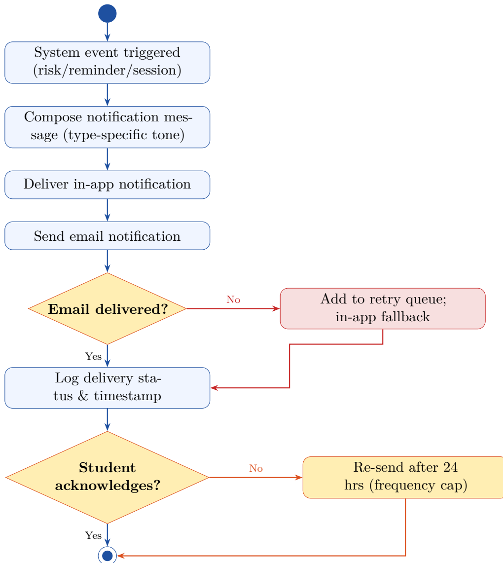
Figure 14: Activity Diagram — UC-06: Receive Notifications &amp; Alerts
