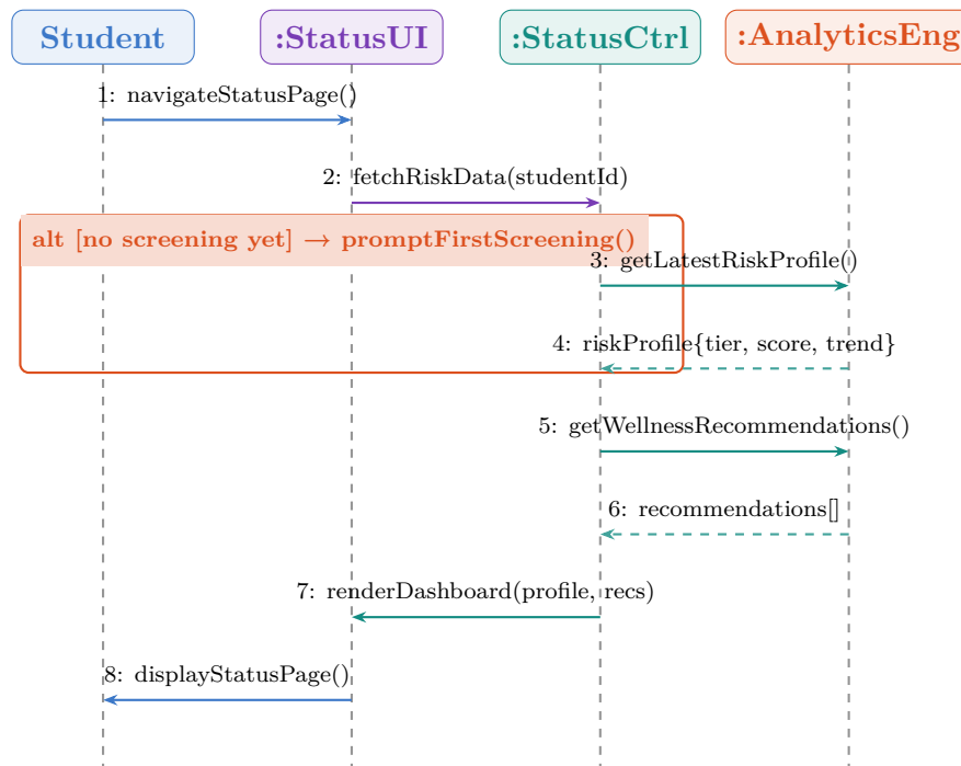
Figure 7: Sequence Diagram — UC-04: View Mental Health Status
