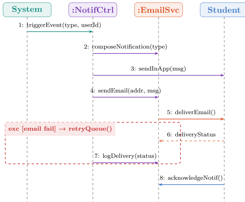
Figure 12: Sequence Diagram — UC-06: Receive Notifications &amp; Alerts
