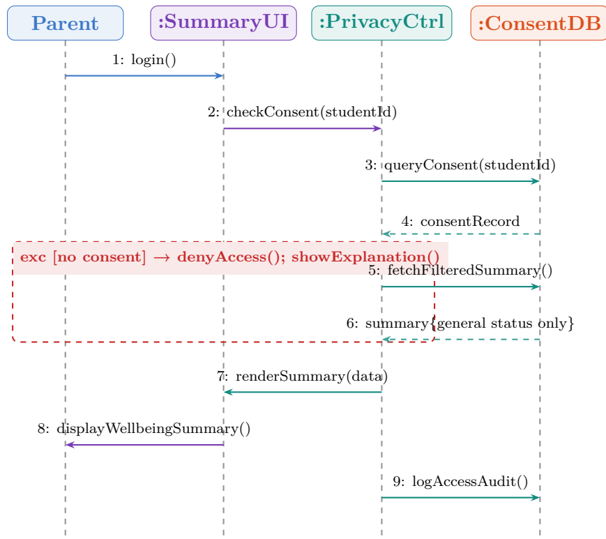
Figure 16: Sequence Diagram — UC-07: View Well-being Summary
