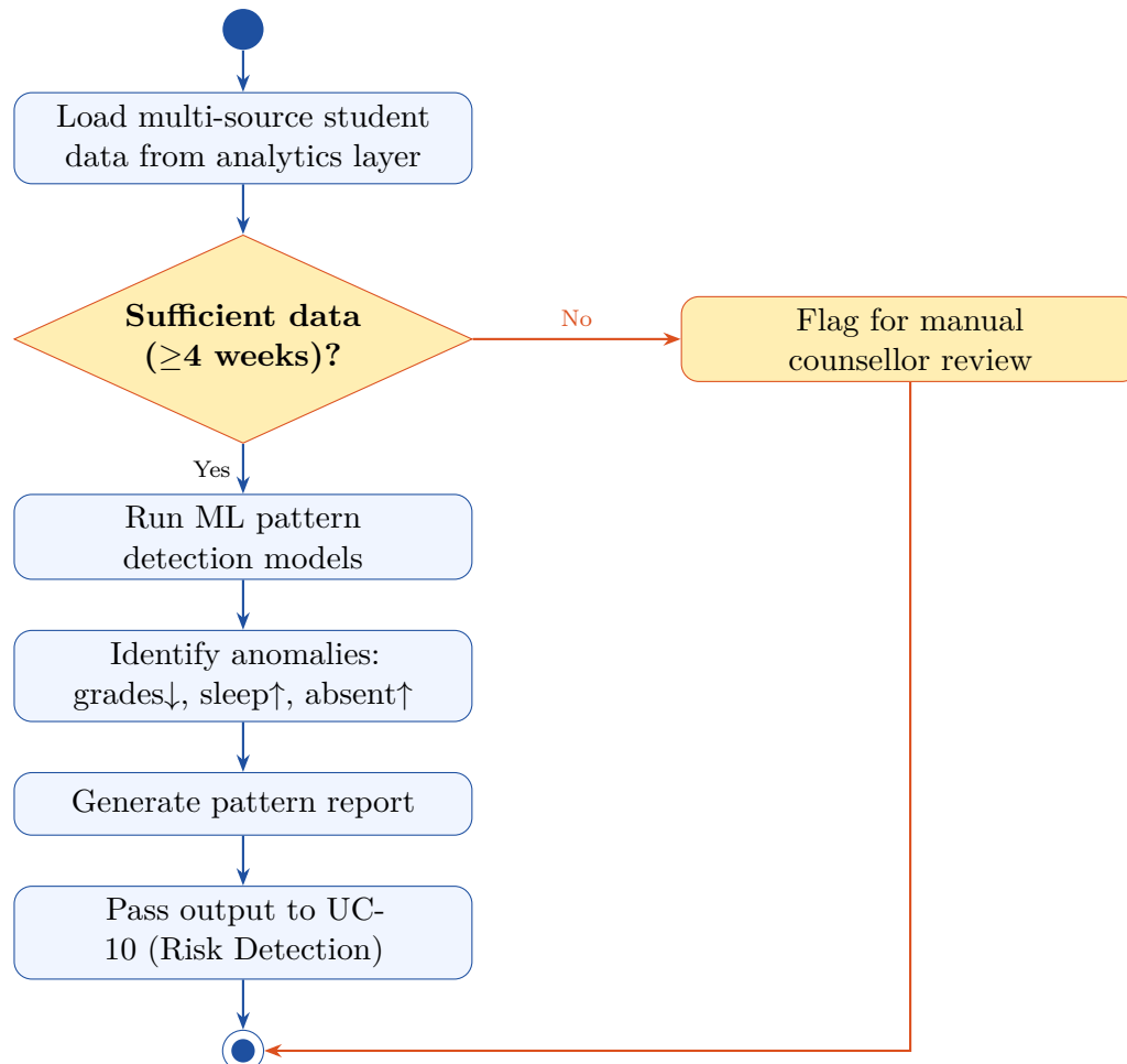
Figure 23: Activity Diagram — UC-09: Analyse Behavioural Patterns
